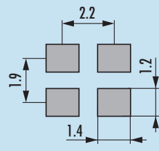
pad layout
