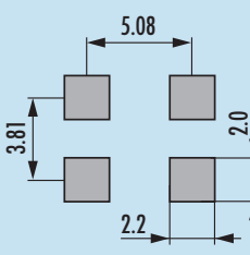
pad layout
